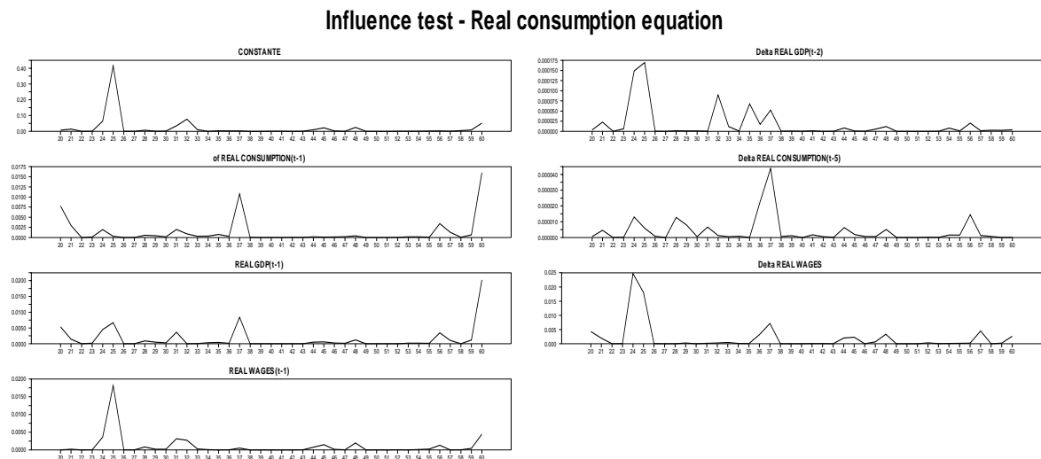
Figure 4.1.4 - Influence test for the coefficients
