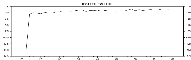
Figure 4.5.3 – Harvey and Collier Phi-test
