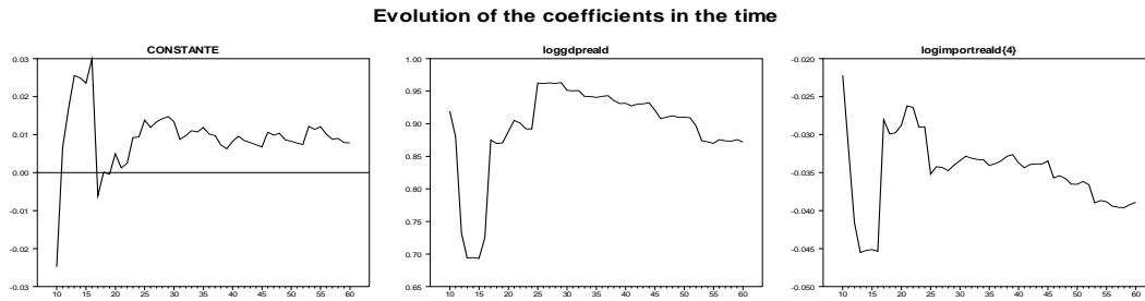
Figure 4.4.1 – Evolution of the coefficients over time
