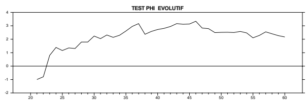
Figure 4.3.3 – Harvey and Collier Phi-test
