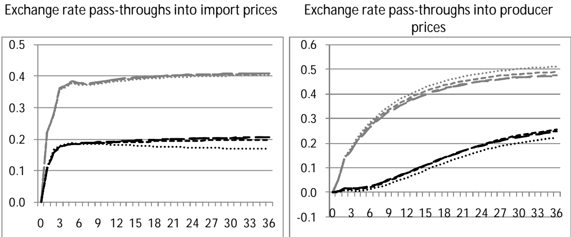
Figure 5. Robustness analysis to the smoothing parameter
