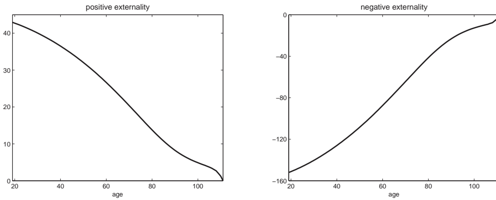
Figure 6: \Theta -term
