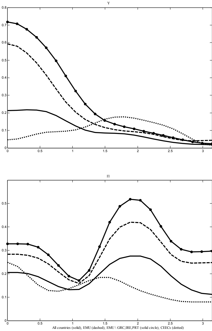
Figure 2: Cohesion 1)
