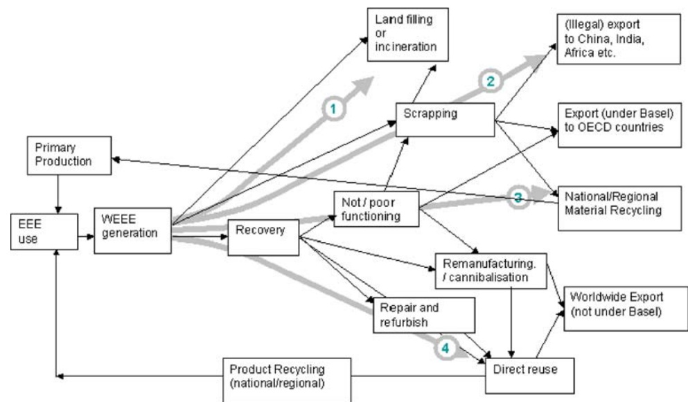
Fig. 2 Flow scheme of national/regional WEEE generation and processing
