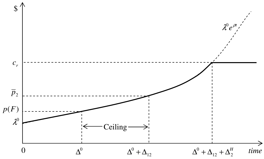
Fig.6. Resource Prices when Natural Gas is Abundant
