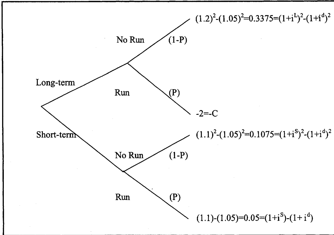
Figure 2: Payoff Tree
