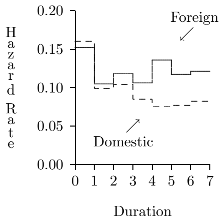
Figure 2: Baseline Hazard Rates
