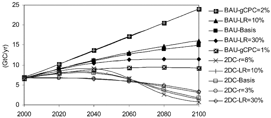
Figure 1. Carbon-dioxide emissions.
