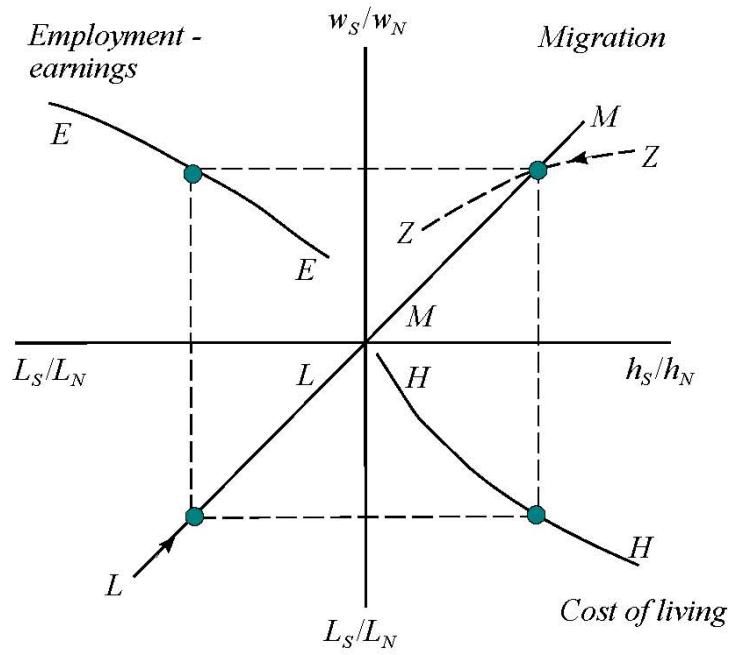
Figure 2: Competing regions
