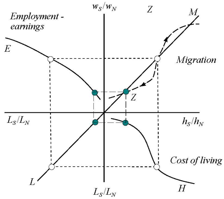
Figure 3: Divergent regions
