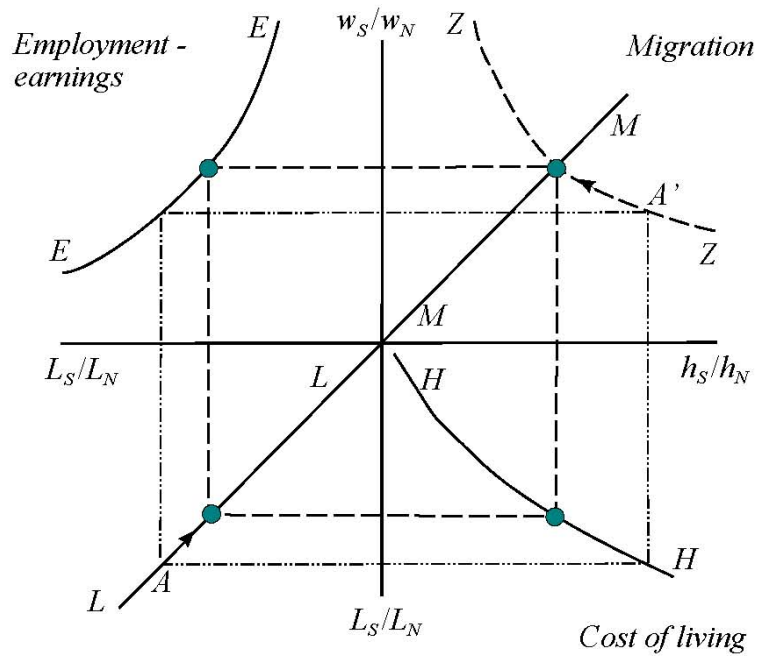
Figure 1: Complementary regions
