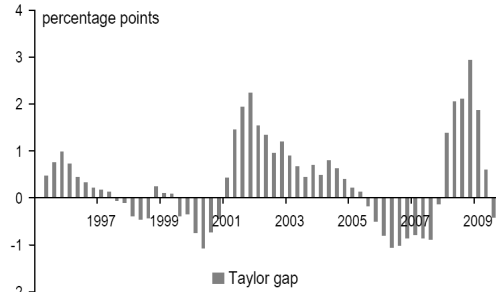
Figure 8: Taylor gap
