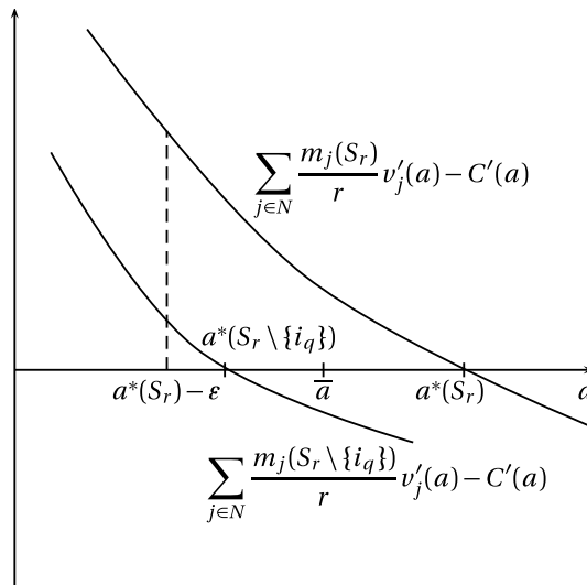
FIGURE 2. Convergence of a^*(S_r \setminus \{i_q\}) to a^*(S_r) .
