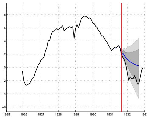
Figure 23: Forecasting the German real sector from March 1931, May 1931 and July 1931, using German and U.S. real variables. The dark gray shaded area represents 68% and the light shaded area 90% of the posterior probability mass.
