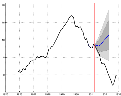
Figure 27: Forecasting the U.S. real sector from March 1931, using U.S. real, banking, and monetary variables. The dark gray shaded area represents 68% and the light shaded area 90% of the posterior probability mass.
