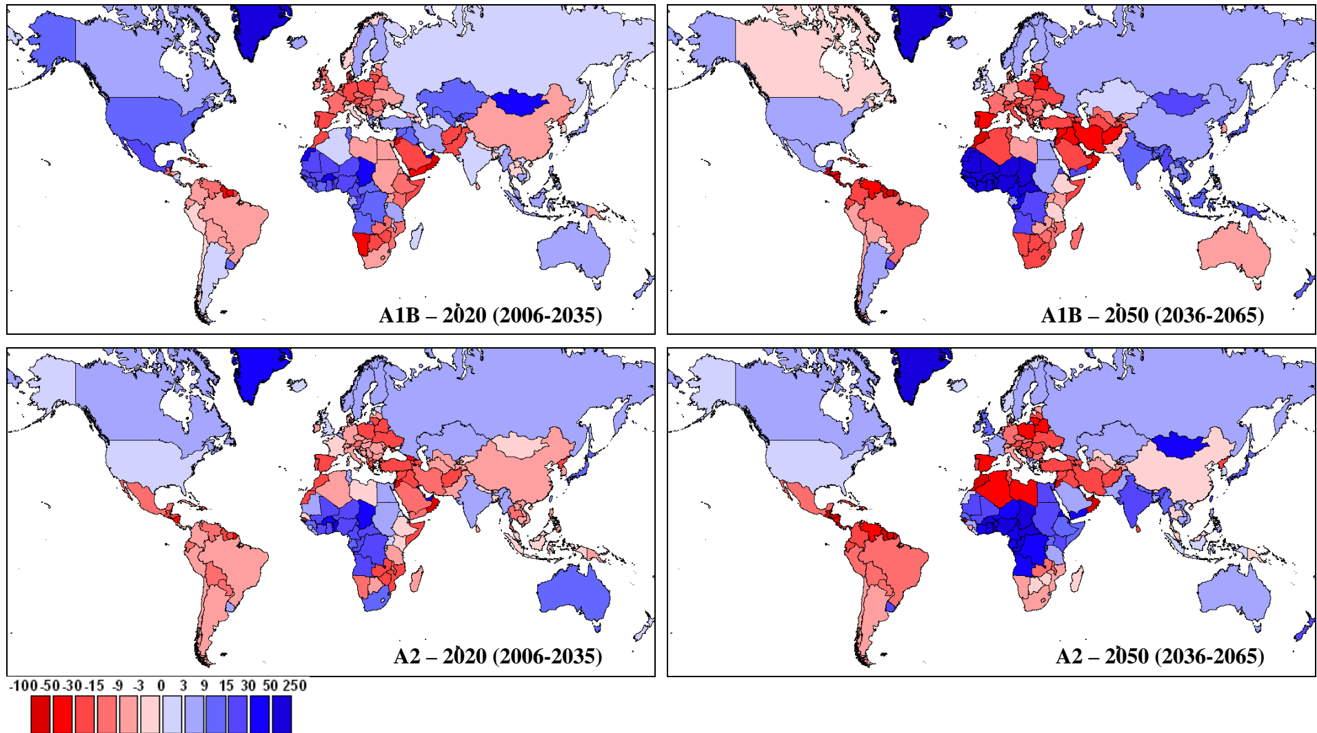
Figure 1. Percentage change in annual average river flow under the two emission scenarios and for the two time periods, with respect to the 30-year average for the 1961-1990 period (historic-anthropogenic simulation)
