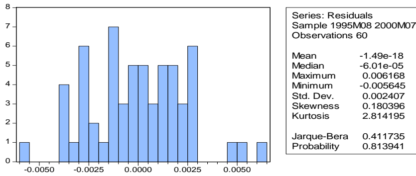
Regression 3
