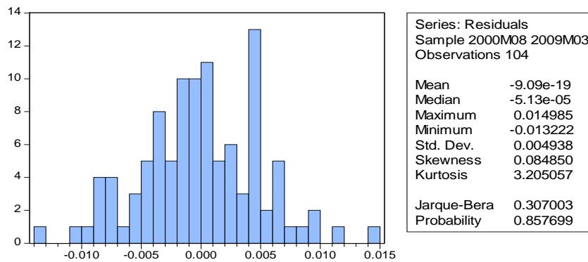
Regression 3
