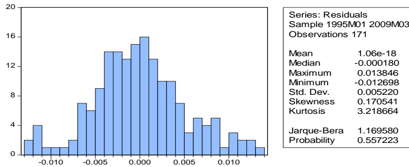
Regression 2
