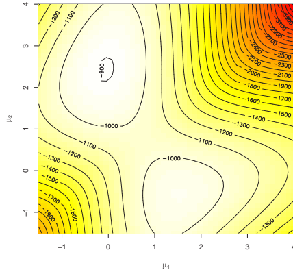
FIGURE 4. R image representation of the log-likelihood of the mixture (1.7) for a simulated dataset of 500 observations and true value (\mu_1, \mu_2, p) = (0, 2.5, 0.7) .
