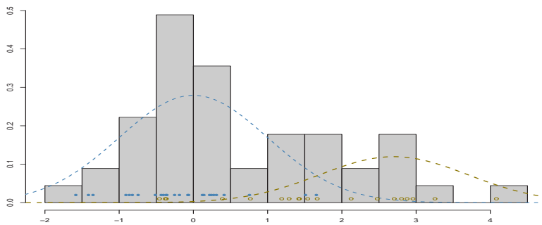
FIGURE 7. Histogram, true components, and most likely allocation found over 440,000 simulations of z 's for a simulated dataset of 45 observations and true values as in Figure 5. Full dots are associated with observations allocated to the first component and empty dots with observations allocated to the second component.
