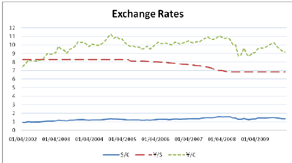
Figure 2. Movements of exchange rate pairs between €, $ and ¥: 2002-2010
