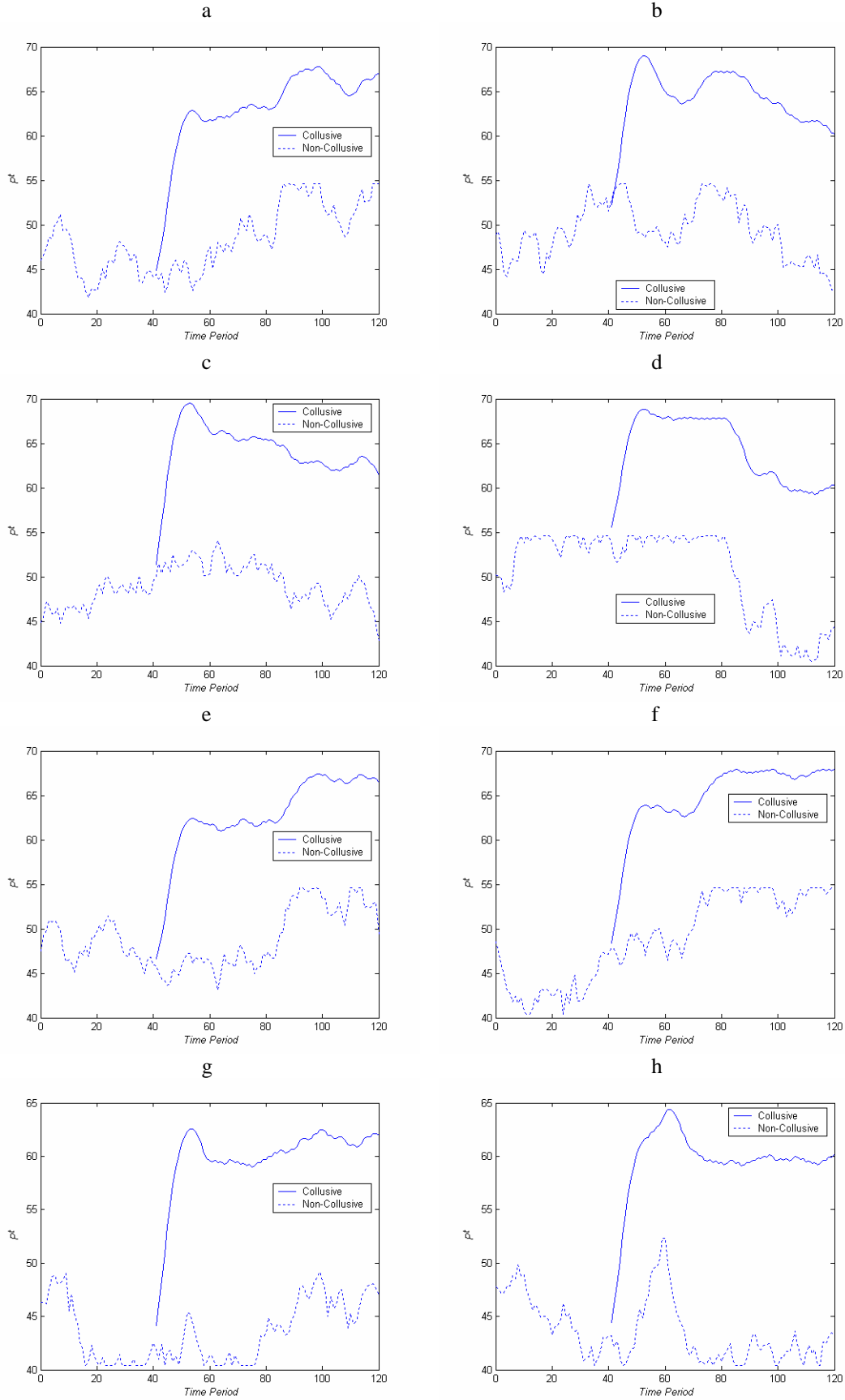
Figure 3. (\xi, \lambda) = (.25, .25)
