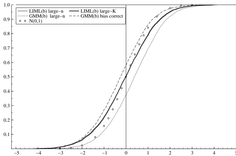
Figure 4: \gamma_{11} : N = 100 , T = 50 , c_b = \frac{4}{100} , (\omega_{11}, \omega_{12}) = (1.0, 0.3)
