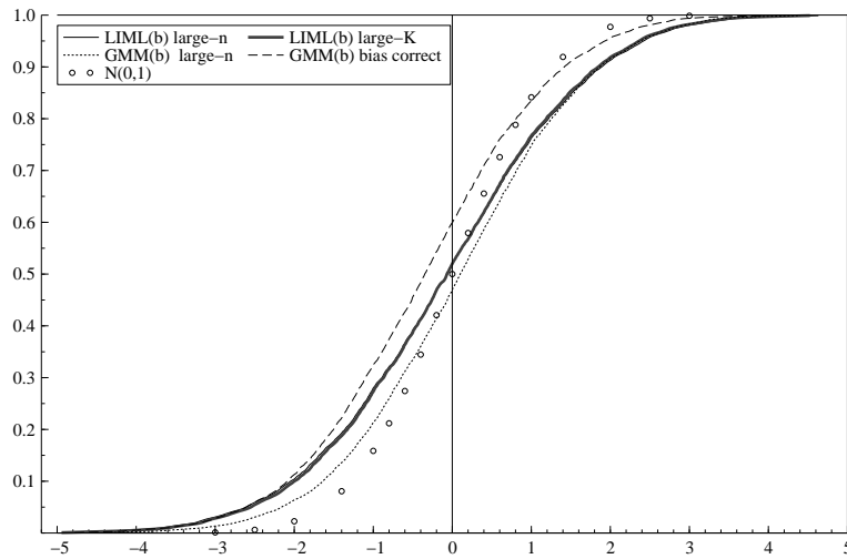
Figure 2: \gamma_{11} : N = 100 , T = 25 , c_b = \frac{4}{100} , (\omega_{11}, \omega_{12}) = (1.0, 0.3)
