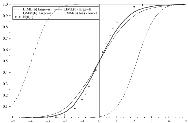
Figure 8: \gamma_{11} : N = 100 , T = 50 , c_b = \frac{4}{100} , (\omega_{11}, \omega_{12}) = (1.5, 1.0)
