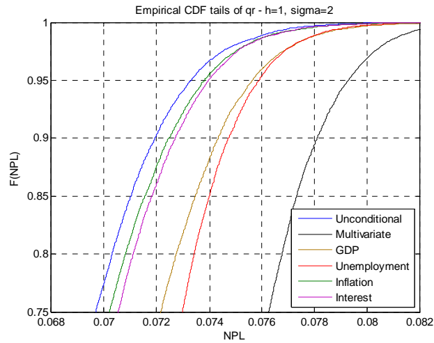
Figure 9 – QR distressed NPL cumulative distribution tails - H=1, \sigma=2
