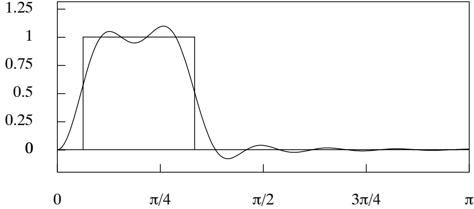
Figure 1. The frequency response of the truncated bandpass filter of 23 coefficients superimposed upon the ideal frequency response. The lower cut-off point is at \pi/16 radians ( 11.25^\circ ), corresponding to a period of 32 quarters, and the upper cut-off point is at \pi/3 radians ( 60^\circ ), corresponding to a period of the 6 quarters.
