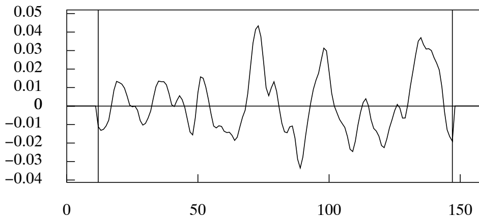
Figure 3. The sequence derived by applying the truncated bandpass filter of 23 coefficients to the quarterly logarithmic data on U.K. Consumption.
