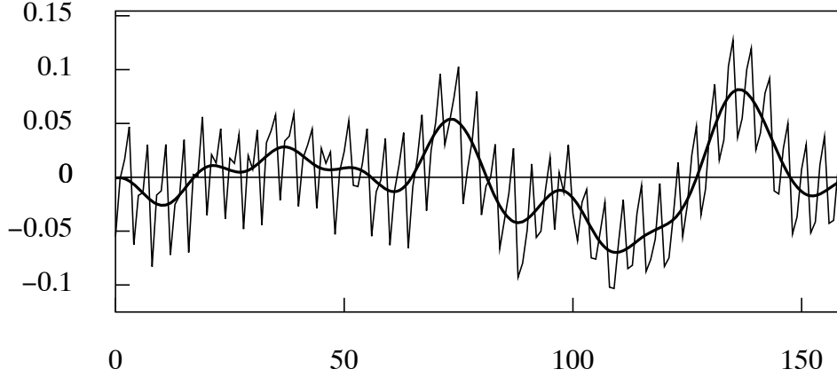
Figure 12. The residual sequence from fitting a quadratic trend to the logarithmic consumption data with an interpolated line representing the business cycle.
