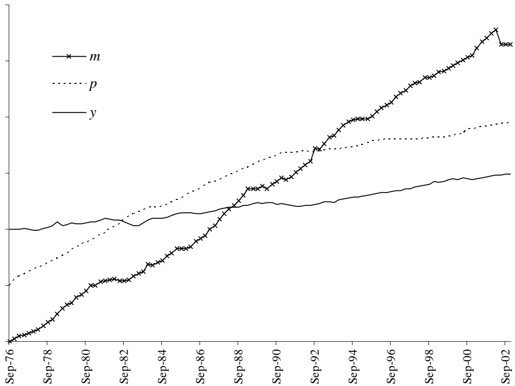
Figure 1: Plot of quarterly log M1, m , price level, p , and real gross national income, y . The sample is from September 1976 to December 2002.
