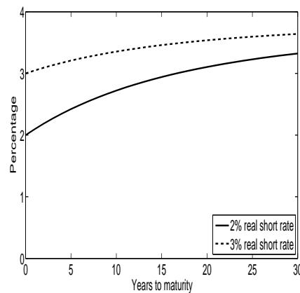
Figure 2.1 – Term structures of real interest rates (in percentages), generated by a one-factor Vasicek model with parameters given in Table 2.5 in Appendix 2.B.
