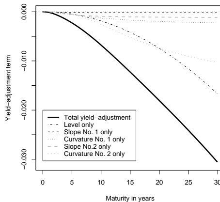
(b) Yield-adjustment in the AFGNS model.
