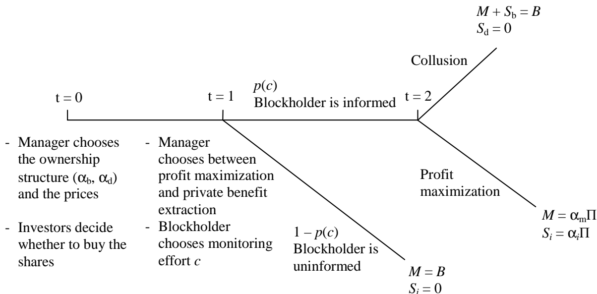
Figure 1: The game.
