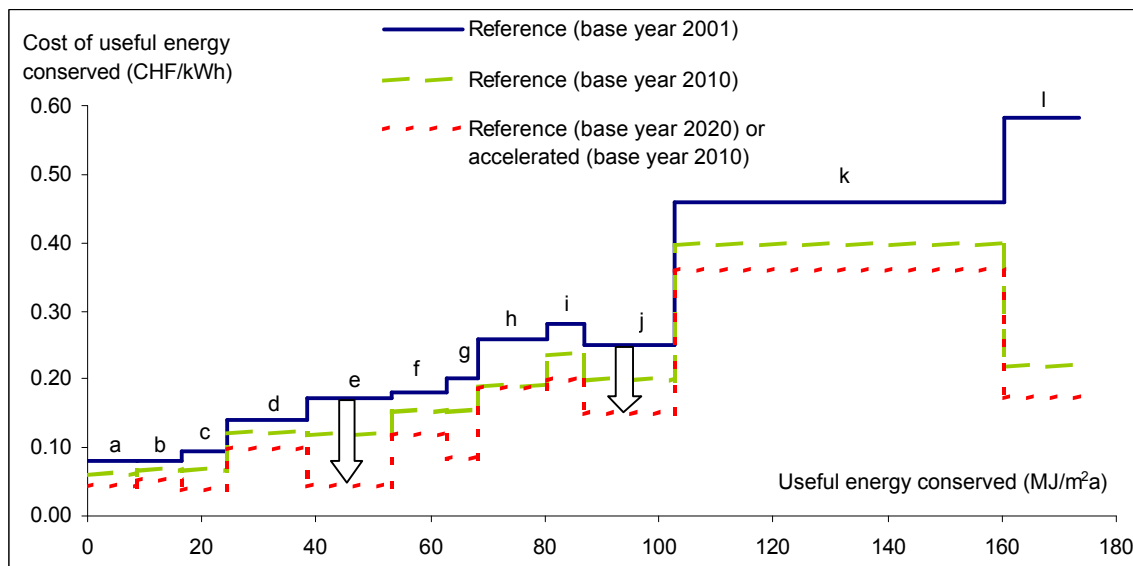
Figure 3 Marginal costs of energy efficiency measures/technologies in relation to the achievable energy efficiency gains for the construction of a new ordinary oil-heated multi-family house in Switzerland, current cost and future or 'enforced' price paths.
