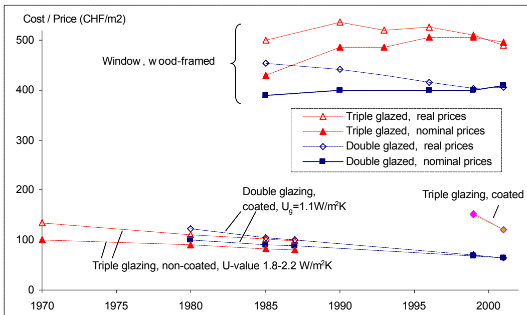
Figure 8 Cost dynamics for window glazing and for standard size wooden frame windows in Switzerland, 1970/1985–2000 (in real 2000 prices)
