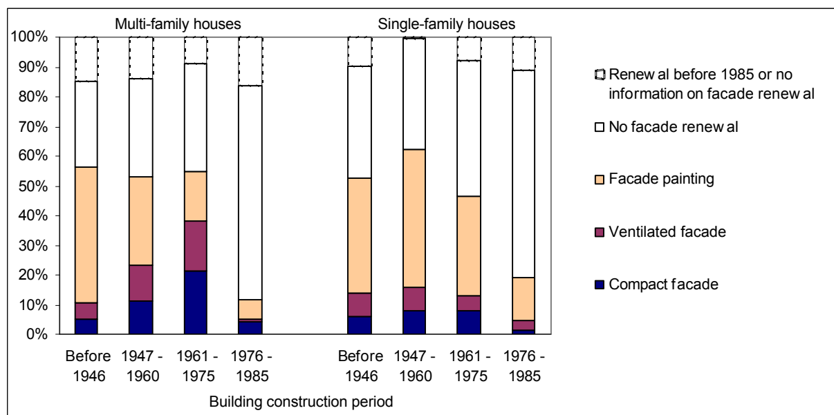
Figure 1 Renewal of residential houses’ façades in Switzerland, 1986-2001 (in %)
