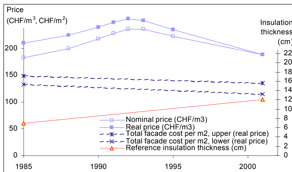
Figure 5 Historical price trajectories for compact façade heat insulation made of polystyrene cellular plastics versus reference wall insulation thickness since 1985, Swiss Canton of Zurich (nominal and real 2000 prices)
