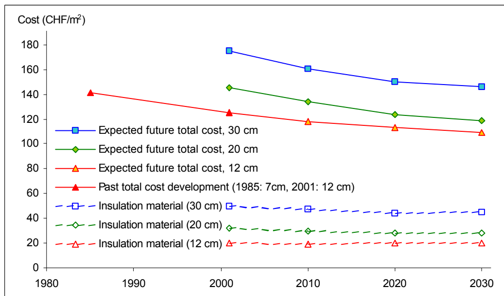
Figure 11 Difference costs for various insulation thicknesses (12, 20, and 30 cm), insulation material alone and total
