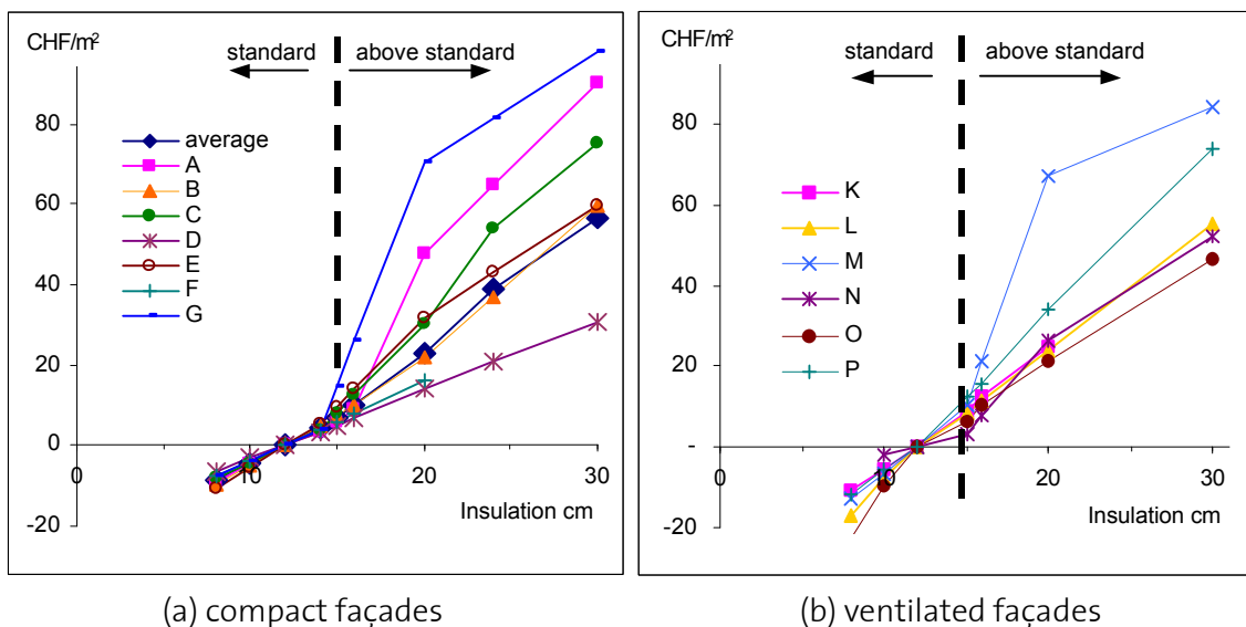
Figure 9 Prices for various wall insulation thicknesses charged by different Swiss building companies (tagged A-P)
