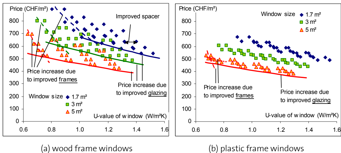
Figure 10 Prices for (a) wood-frame and (b) plastic-frame windows in Switzerland as a function of window-U-values for various frame and glass qualities, various spacers and window sizes (1.7 m 2 , 3 m 2 , and 5 m 2 ; frame shares 30%, 22%, and 15%)
