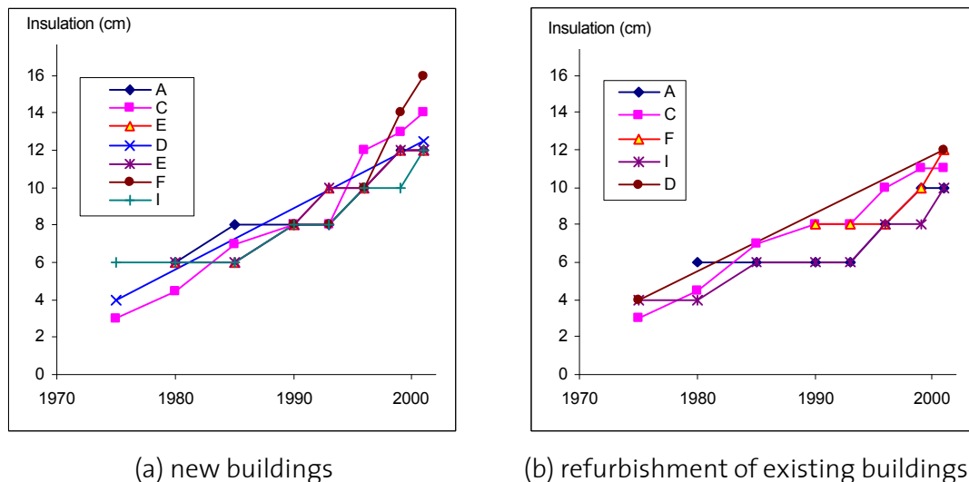
Figure 4 Thickness of the standard building envelope insulation (case of ventilated facades) applied by various Swiss companies, 1970-2001
