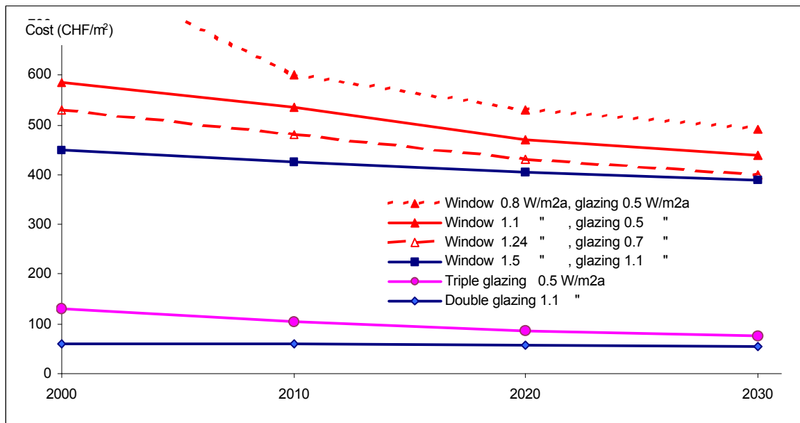
Figure 12 Estimated costs for windows and various glazing qualities, single glazing (various U-values), double and triple glazing, 2000-2030
