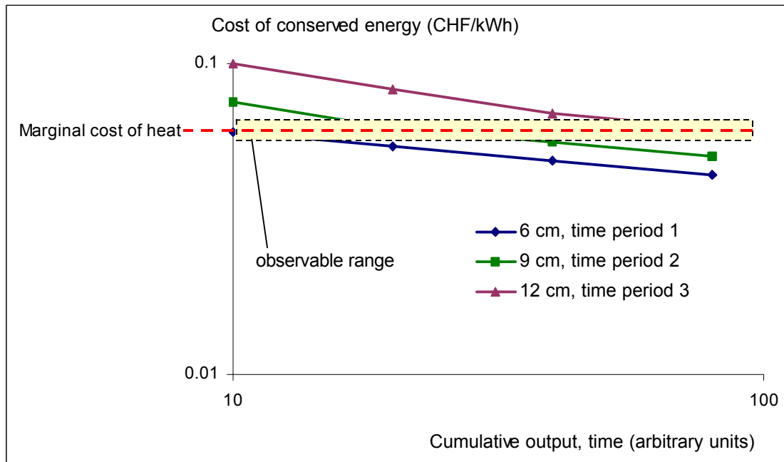
Figure 2 Experience curves for different insulation thicknesses versus marginal cost of heating (stylised)
