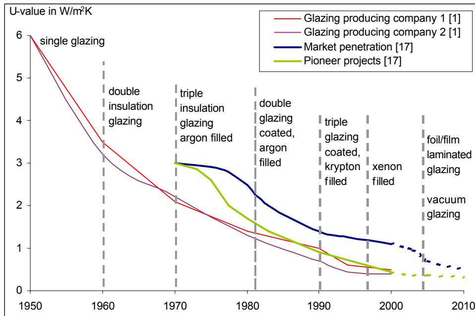
Figure 7 Development of the U-values of window glazing (i.e. w/o frames) from 1950-2000 and possible future development scenario until 2010, and approximate market introduction of various window glazing technologies
