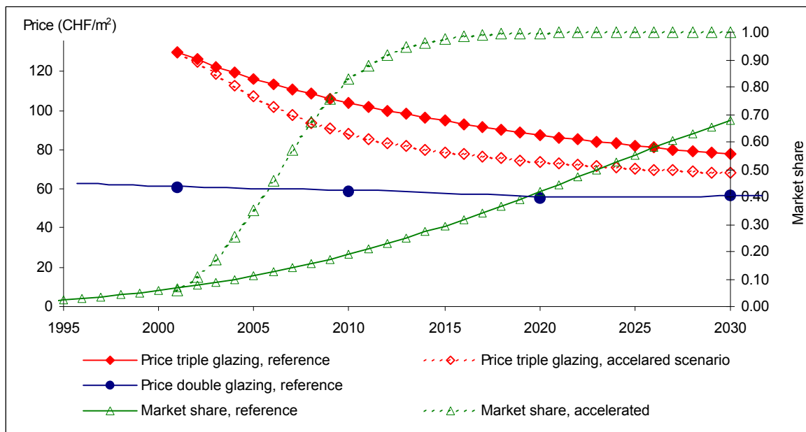
Figure 13 Price development paths for different assumptions on market shares for triple glazed windows, 1995-2030 (simulation)
