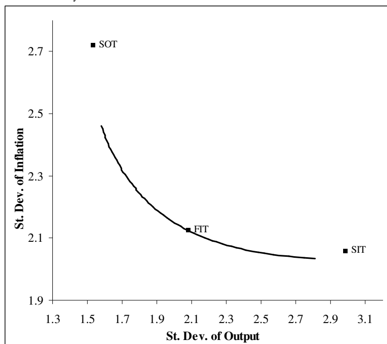
Figure 3: Efficiency Frontier
