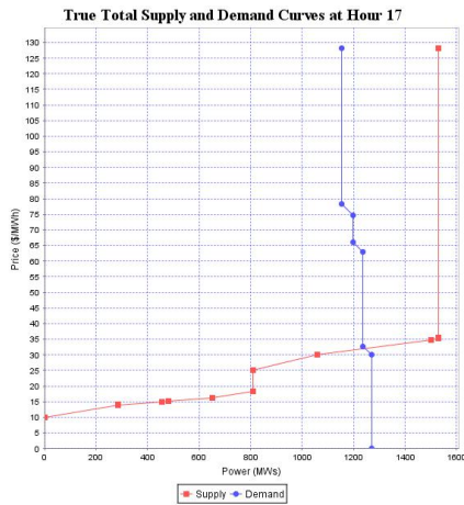
Fig. 6. True total supply and demand schedules during the peak-demand hour 17 of a day-ahead energy double-auction market for a benchmark (no-learning) 5-bus test case explored in [7] using the AMES Test Bed.
