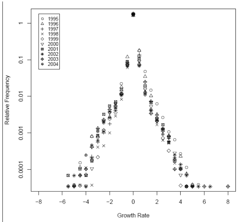
Figure 1: Growth rates distribution, 1995-2004
