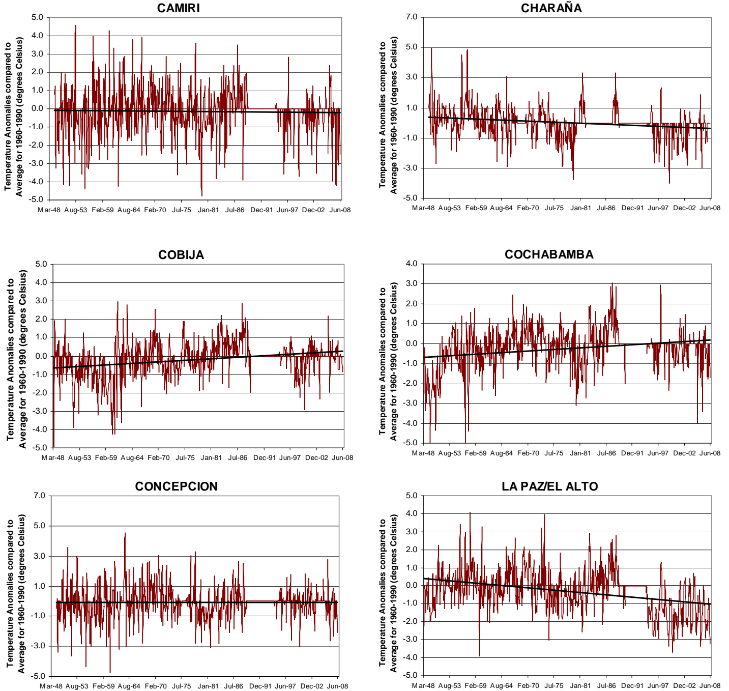
Figure A1: Monthly temperature anomalies for 18 meteorological stations in Bolivia, 1948-2008
