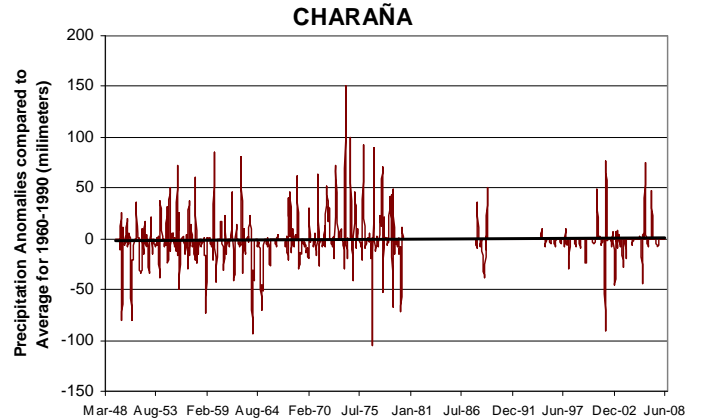
Figure A2: Monthly precipitation anomalies for 19 meteorological stations in Bolivia, 1948-2008
