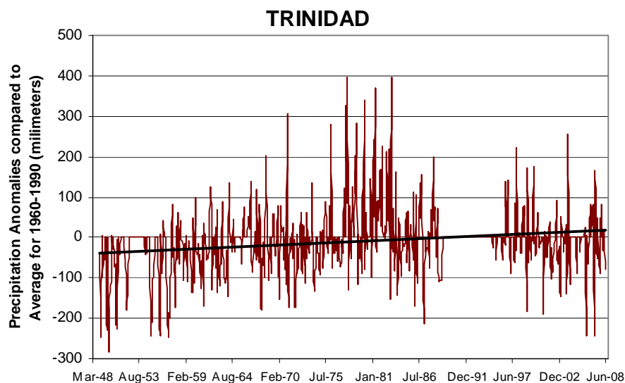
Figure 3: Trinidad: average monthly precipitation anomaly, 1948-2008, compared to average monthly precipitation for 1960-90.
