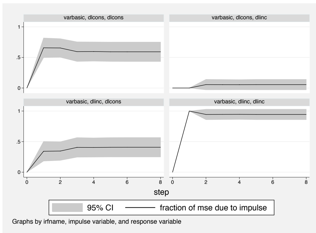
Figure 5: Forecast error variance decomposition of differenced natural logged consumption and differenced natural log of income, using Lütkepohl (1993) West German economic data.
