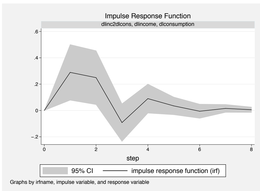
Figure 2: Impulse response function from a univariate dynamic regression model of differenced natural log of consumption as a response to a unit impulse in the differenced natural log of income, using Lütkepohl (1993) Table E1: West German macroeconomic data.
