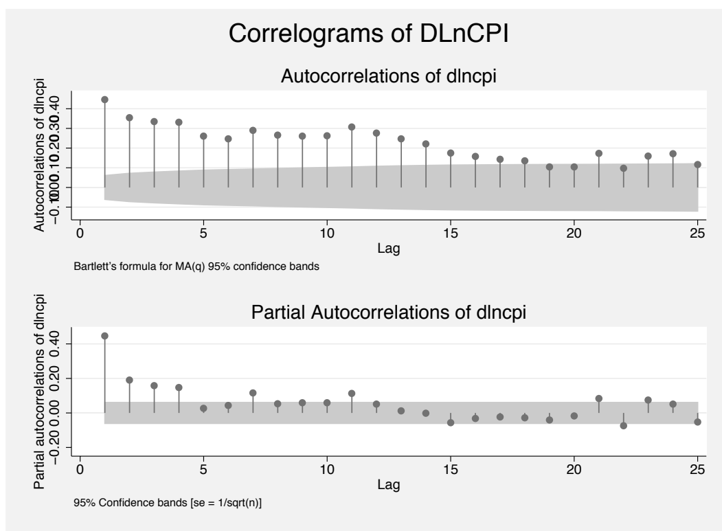
Figure 1: Combined correlograms.
