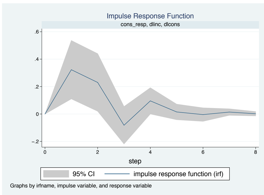
Figure 4: Orthogonalized impulse response functions of differenced natural log of consumption and differenced natural log of income to unit impulses from the other, using Lütkepohl (1993) West German economic data.
