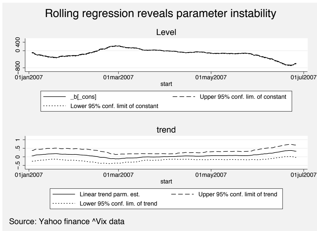
Figure 3: Rolling regression estimates of constant and coefficient in 60-day window.
