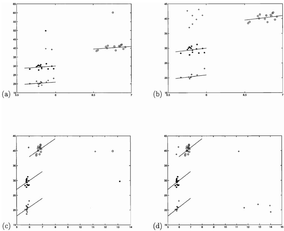
Figure 1: Scatterplot of y_{it} versus x_{it} for 1 \leq t \leq 15 and 1 \leq i \leq 3 . Different time-series are indicated with different symbols. Four cases are considered: (a) only vertical outliers, (b) block concentrated vertical outliers, (c) leverage points, (d) block concentrated leverage points.
