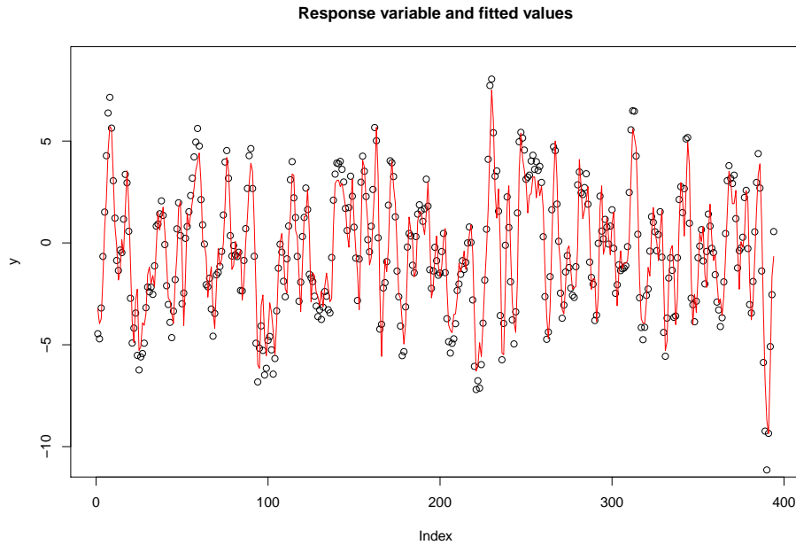
Figure 3: Plot of observations with fitted values from gmm object.
