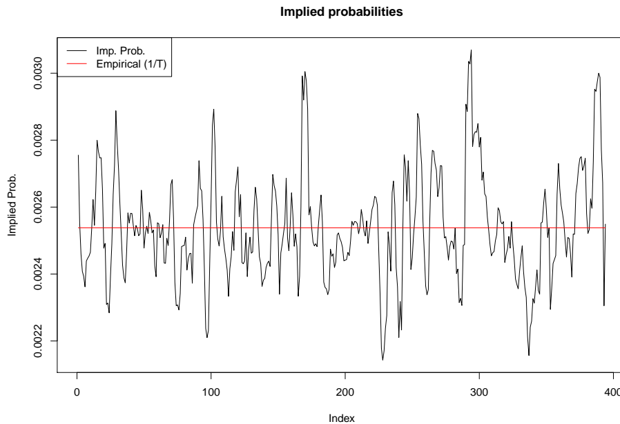
Figure 4: Implied probabilities constructed from the plot function on a gel object.
