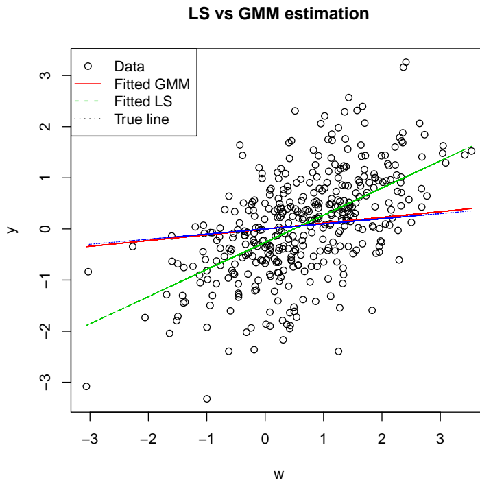
Figure 1: Visual comparison of lm and gmm fits.
