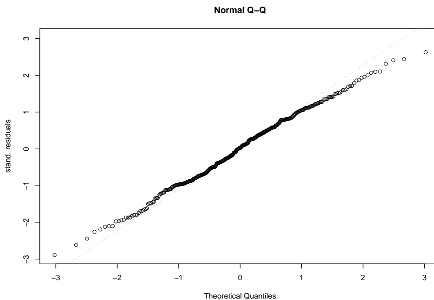
Figure 2: Q-Q plot of the residuals from gmm object.
