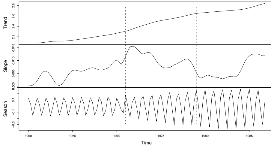
Figure 2: Time-varying trend, slope, and seasonal components in UK gas consumption.
