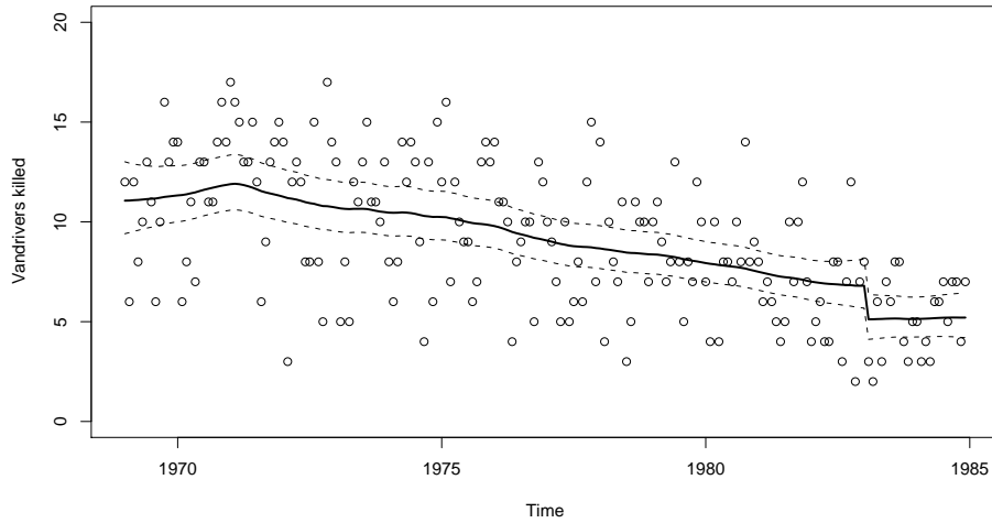
Figure 3: Estimated trend and intervention (solid line) for the vandivers data. The dashed lines are \pm 2 standard deviations.
