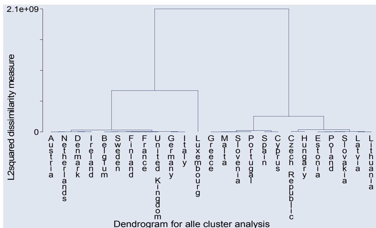
Figure 9 Cluster Analyses: Period: 2000-2003, Wards Method
