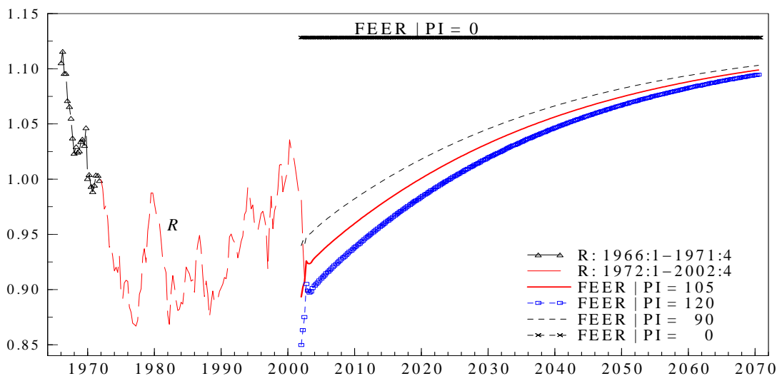
Figure 10: Petroleum wealth and the real exchange rate. Actual observations of the real exchange rate in the period 1966q1–2002q4 together with the simulated paths of the FEER in the period 2002q1–2070q4, see Figure 8 for more details. Given that data for a trade-weighted real exchange rate were not publicly available, observations of the real exchange rate in the period 1966q1–1971q4 are based on import weights while those afterwards are based on trade weights. Source: Norges Bank.
