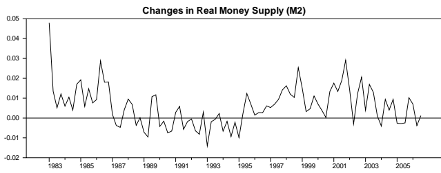
Figure 3: Data in first differences
