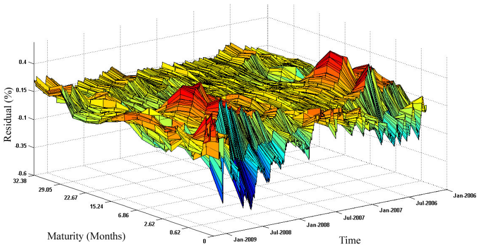
Fig. 4. Residuals of the estimated yield curve (Jan 2006 to Feb 2009)
