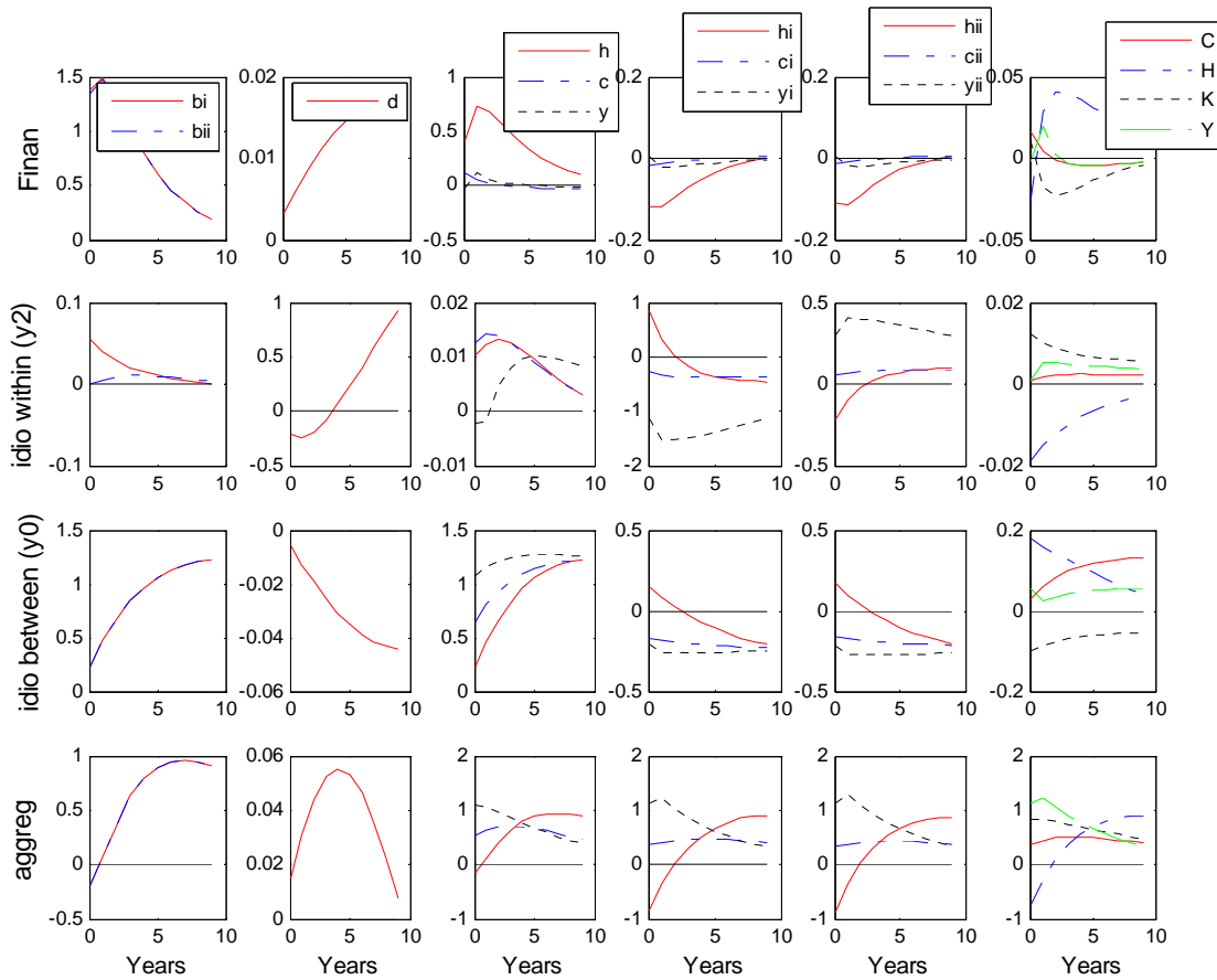
FIGURE 2: Impulse Responses of the model
