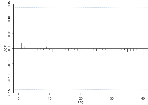
(b) ACF of simulated \text{Var}(D_t)
