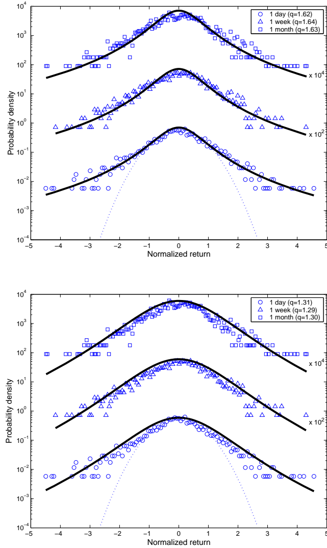
Figure 1: EMPIRICAL HISTOGRAMS FOR THE DAILY, WEEKLY AND MONTHLY S&P-500 INDEX NORMALIZED RETURNS (1990-2000)
