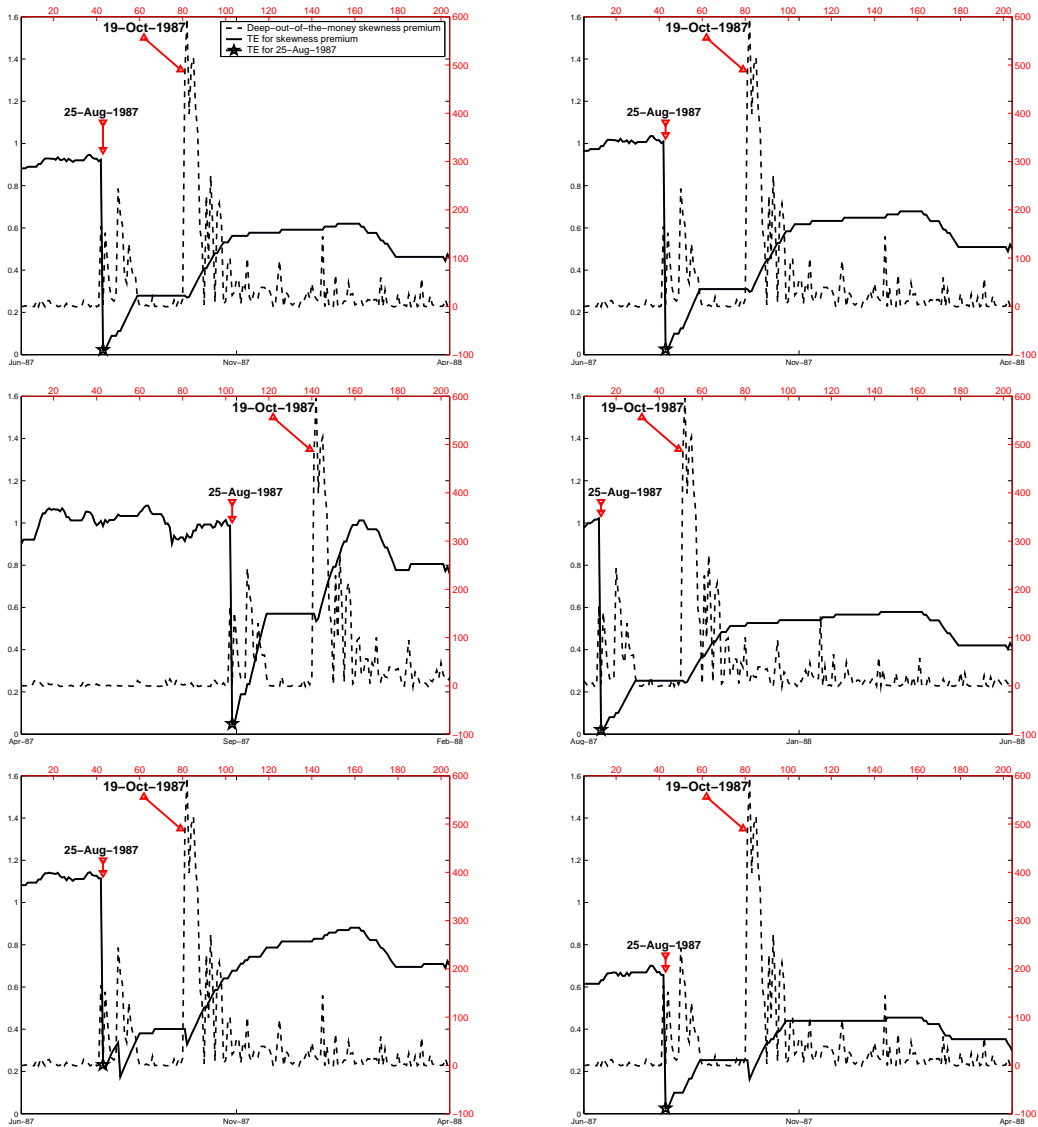
Figure 6: ROBUSTNESS TESTING
