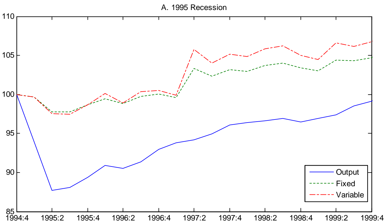
Figure 11 Output and Predictions of Model with No Efficiency Wedge and Two Capital Utilization Specifications
