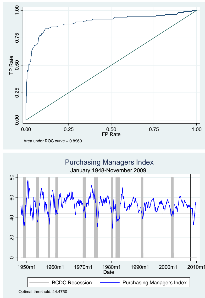
Figure 7. The Purchasing Managers Index (PMI) : ROC Curve and Time Series Plot with Optimal Threshold
