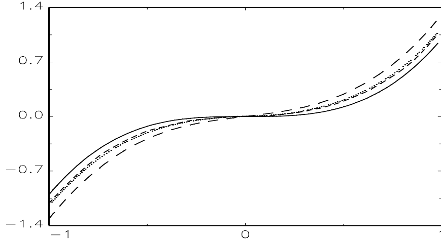
Figure 3: Graphs of f_B(x) and Monte Carlo estimates of E(\hat{f}_B(x)) for h = n^{-1/2} (short dashes), h = n^{-1/3} (dotted) and h = n^{-1/5} (long dashes) with \theta = 100 , \sigma = 0.1 and n = 500 .
