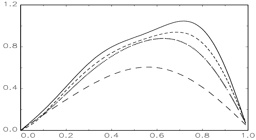
Figure 1: Graphs over the interval [0, 1] of f_A(x) and Monte Carlo estimates of E(\hat{f}_A(x)) for h = n^{-1/2} (short dashes), h = n^{-1/3} (dotted) and h = n^{-1/5} (long dashes) with \theta = 100 , \sigma = 0.1 and n = 500 .
