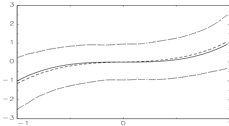
Figure 4: Graphs of estimation bands for f_B(x) (solid line), the Monte Carlo estimate of E(\hat{f}_B(x)) for h = n^{-1/3} (short dashes) and 95% estimation bands (dotted) with \theta = 100 , \sigma = 0.1 and n = 500 .
