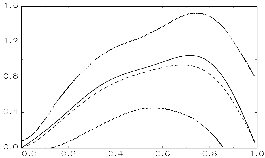
Figure 2: Graphs over the interval [0, 1] of estimation bands for f_A(x) (solid line), the Monte Carlo estimate of E(\hat{f}_A(x)) for h = n^{-1/2} (short dashes) and 95% estimation bands (dotted) with \theta = 100 , \sigma = 0.1 and n = 500 .
