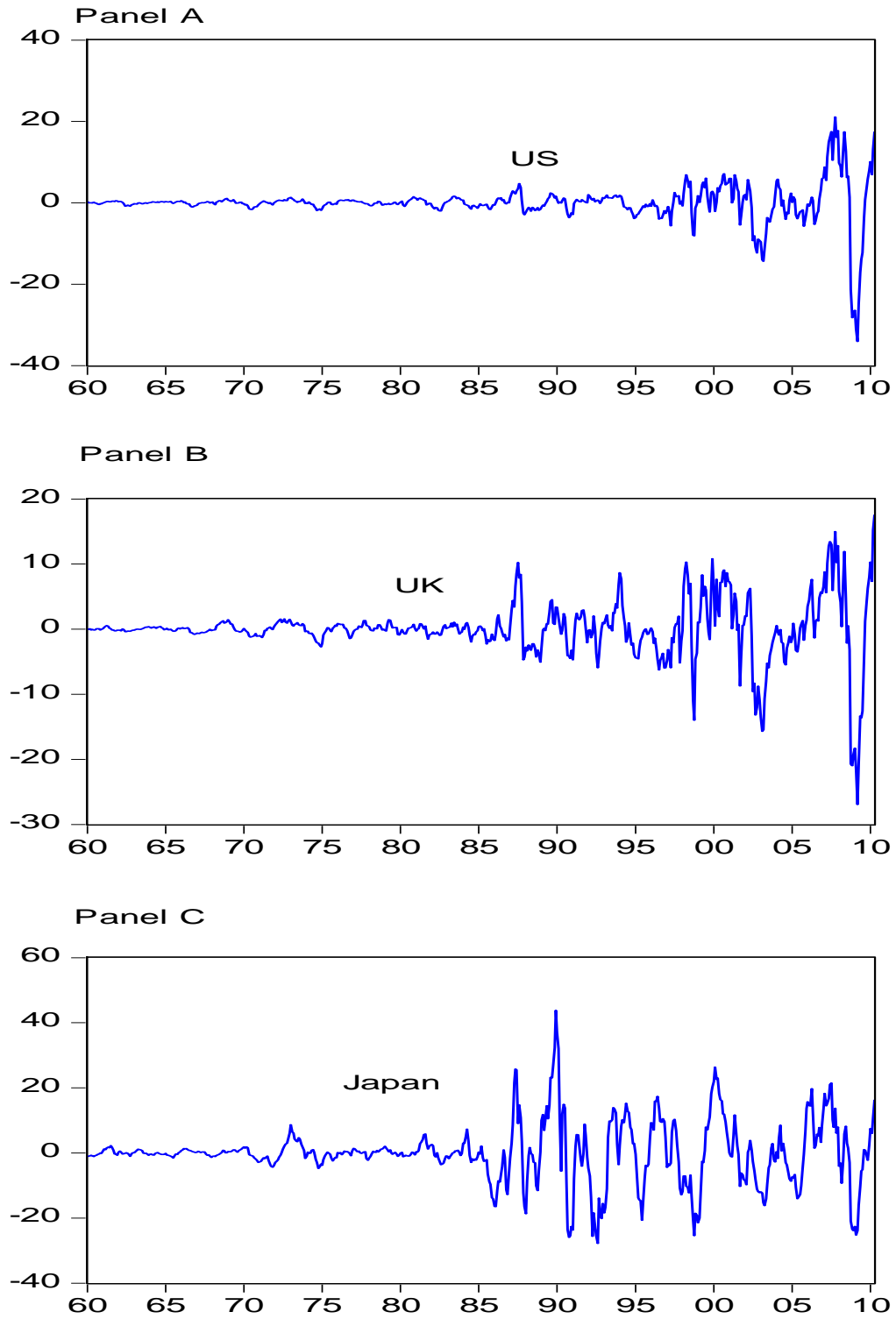
Figure 2: Cyclical components of stock price series for the US, the UK and Japan
