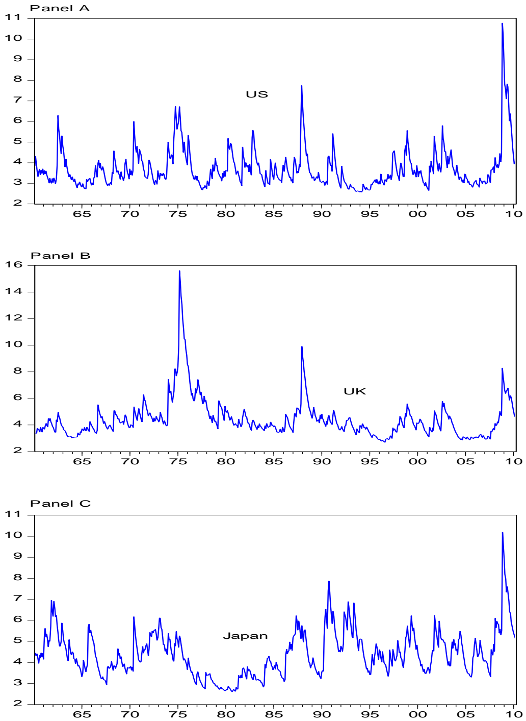
Figure 4: Conditional standard deviation of US, UK and Japan
