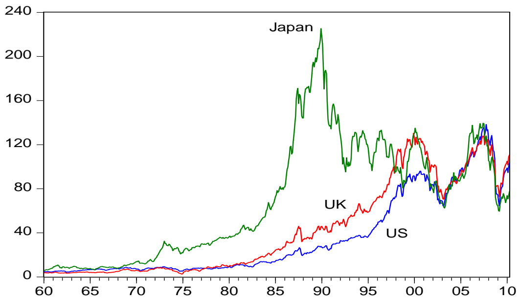
Figure 1: Stock price index of US, UK and Japan
