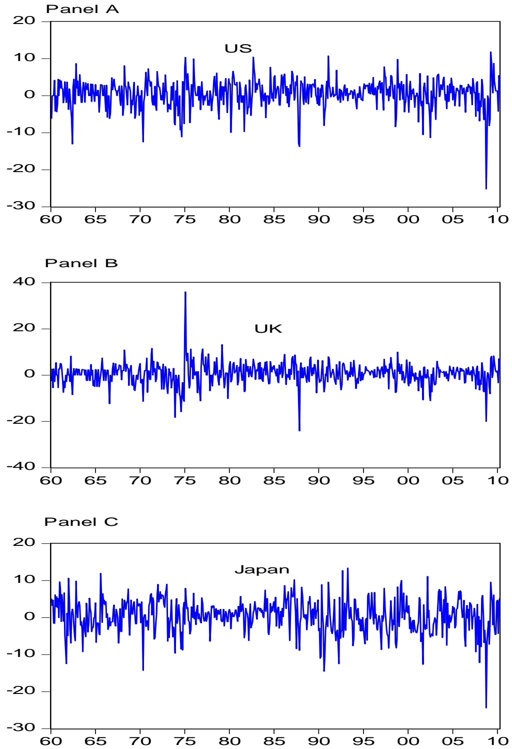
Figure 3: Growth rate of stock prices in US, UK and Japan
