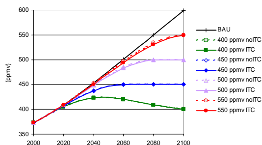
FIGURE 1. Atmospheric CO 2 concentration
