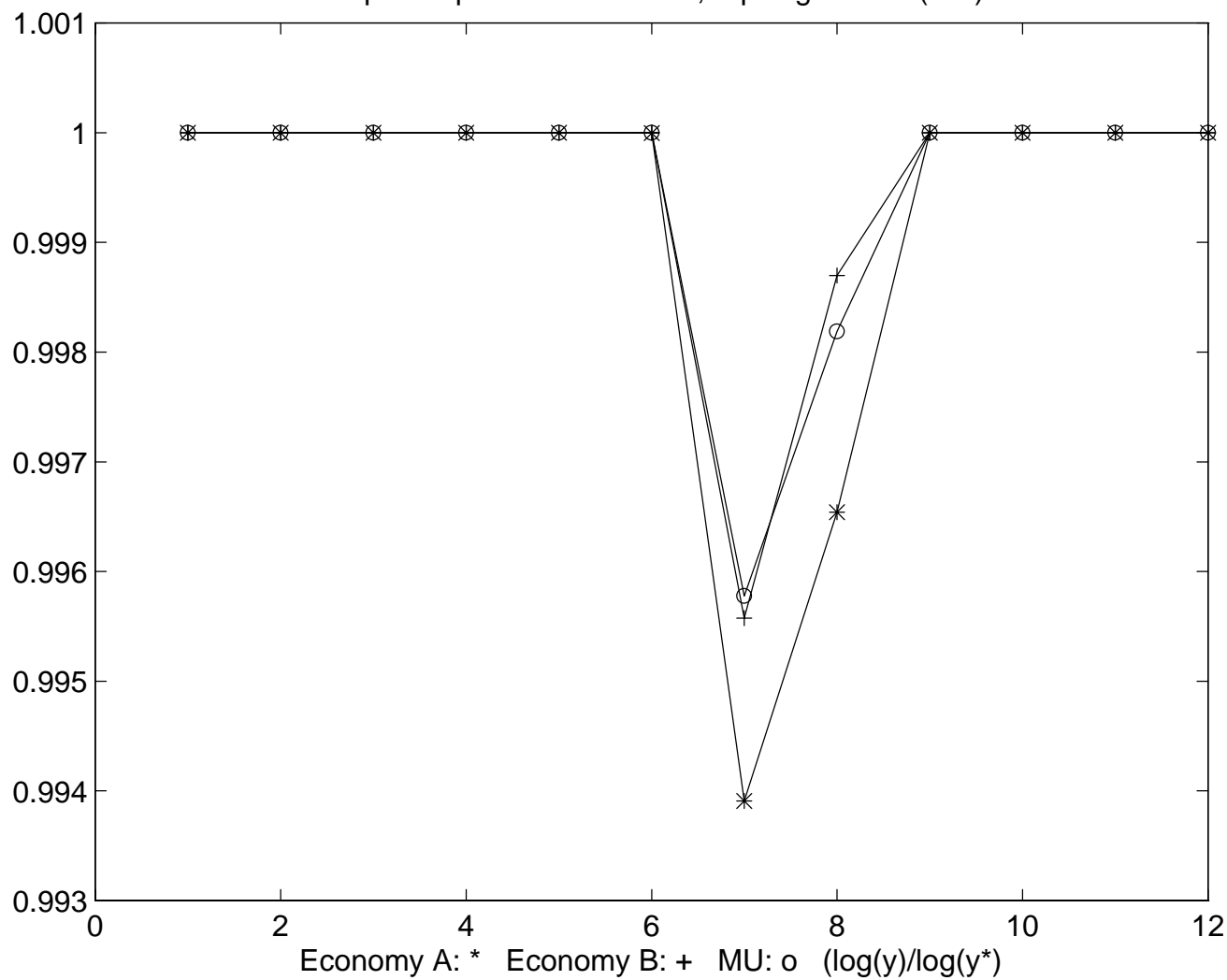
Output resp. to a mon. contr., equal gammas (MU)
