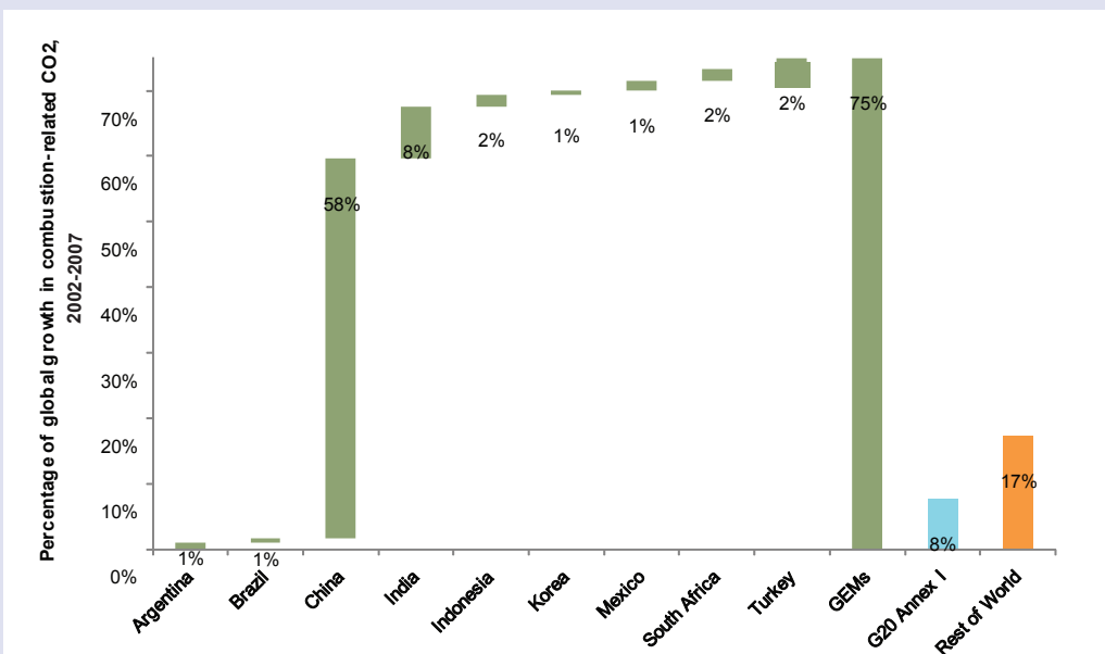
Figure A6 | Three quarters of the growth in combustion related global emissions between 2002 and 2007 came from the GEMs
