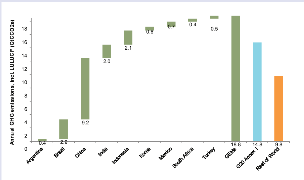
Figure A5 | GEMs account for a greater proportion of current emissions than the G20 Annex 1 countries
