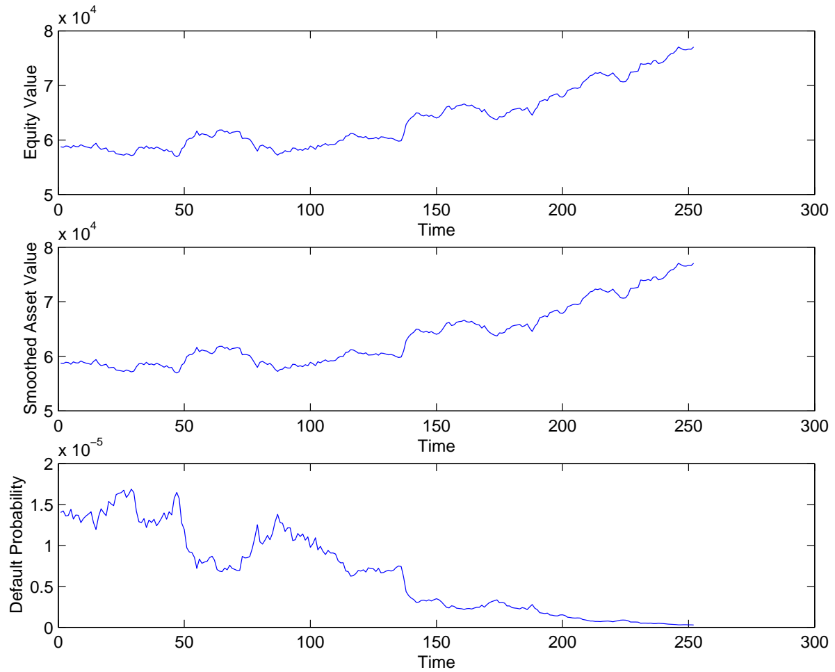
Figure 4: The observed equity values, the smoothed firm asset values and default probabilities of 3M in Mod 1.
