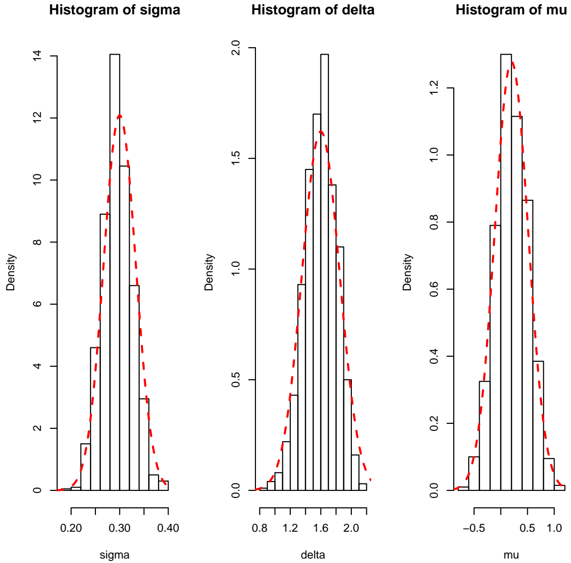
Figure 1: Finite sample distribution (histogram) of MLE of \sigma , \delta (multiplied by 100), \mu based on the particle filtering method of Duan and Fulop (2009). The dotted line is the standard asymptotic distribution where the asymptotic variance is obtained from the Fisher information matrix.
