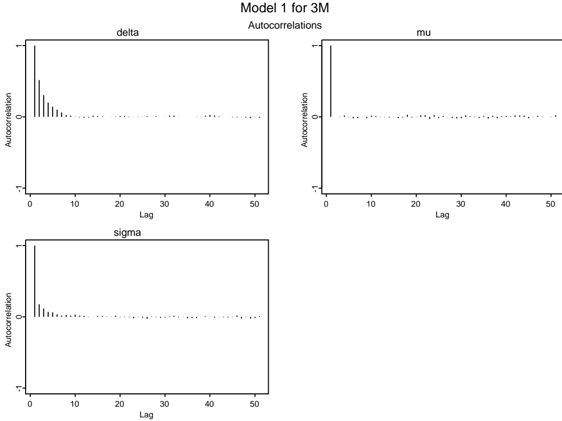
Figure 3: Autocorrelation functions of parameters in Mod 1.
