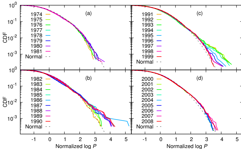
Fig. 9. Cumulative distribution function of normalized log land prices for each year in 1974-1981 (a), in 1982-1990 (b), in 1991-1999 (c), and in 2000-2008 (d). Colors represent different years. The dotted line represents the cumulative distribution function of the standard normal distribution.
